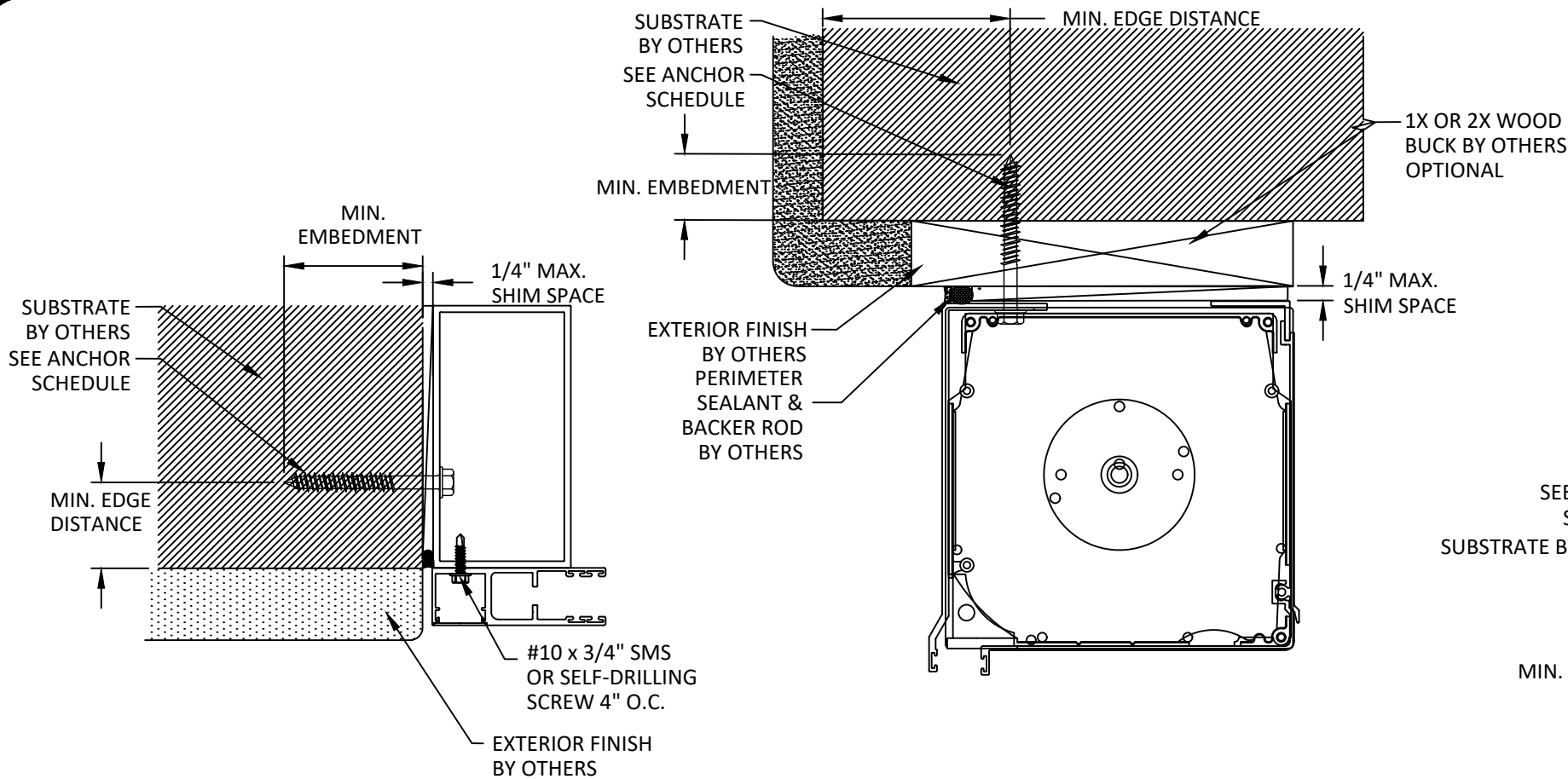
A 5 ANCHOR DETAIL THROUGH FRAME INSTALLATION
