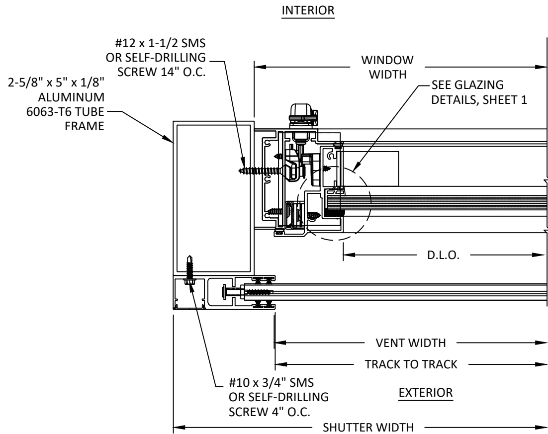
A/4 HORIZONTAL SECTION LEFT JAMB DETAIL
