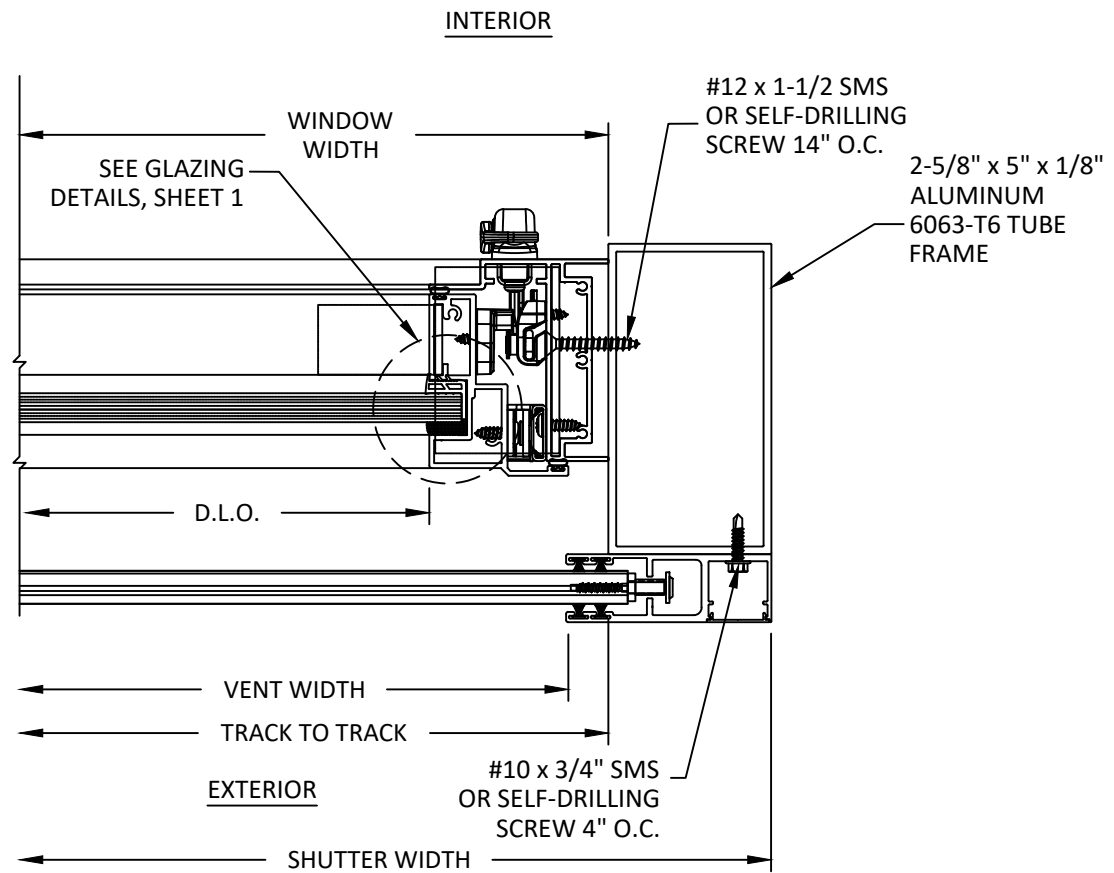
B/4 HORIZONTAL SECTION RIGHT JAMB DETAIL
