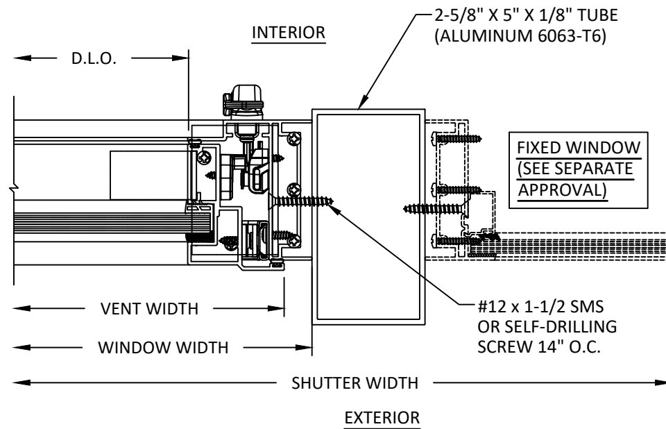
D/4 HORIZONTAL SECTION PROJECT OUT TO FIXED
