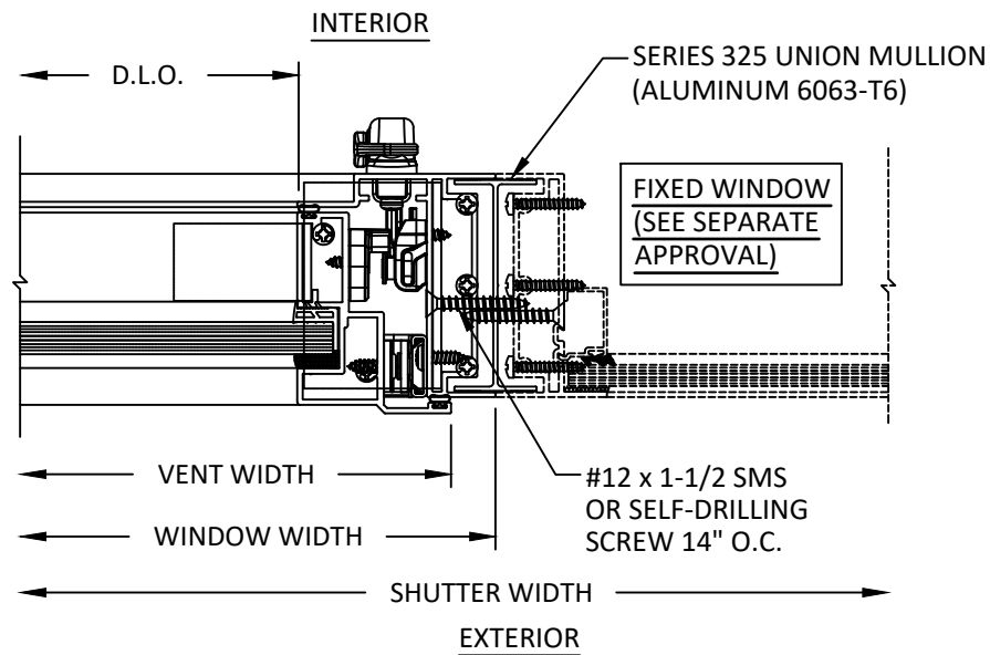
C/4 HORIZONTAL SECTION PROJECT OUT TO FIXED
